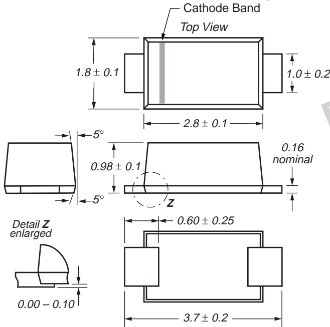
DO-219 (SMF)
