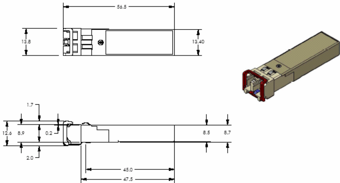
Figure 4: Package Outline Drawing (with Thumb-Release (Button) Latch)
