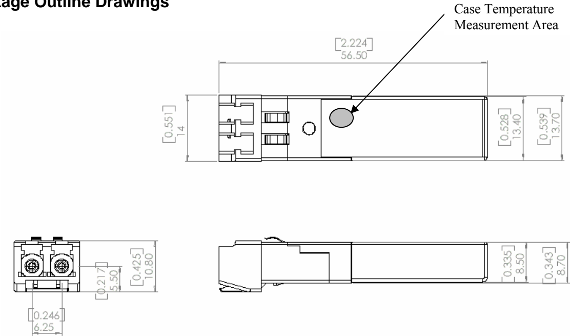
Figure 4: Package Outline Drawing (with Thumb-Release (Button) Latch)
