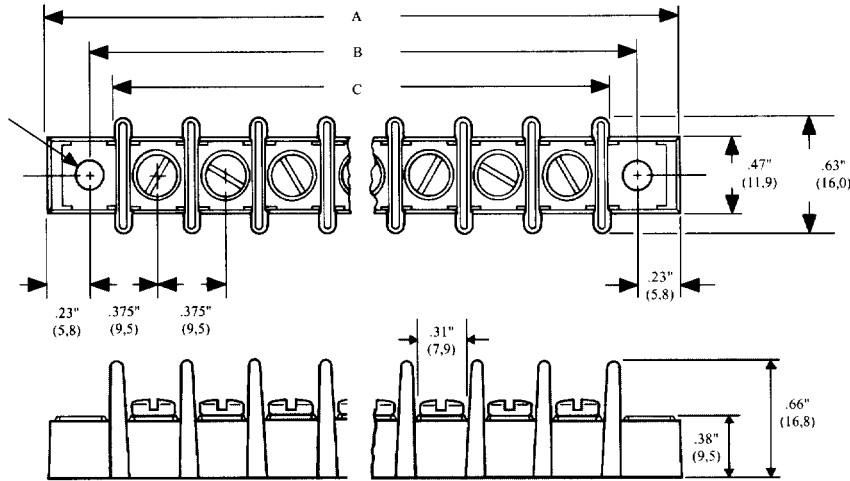
Solid Mounting Ends
