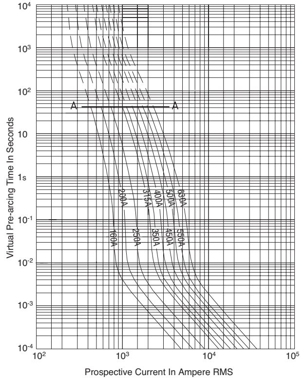
Size 1 — 160-630A: 1000V Time-Current Curve
