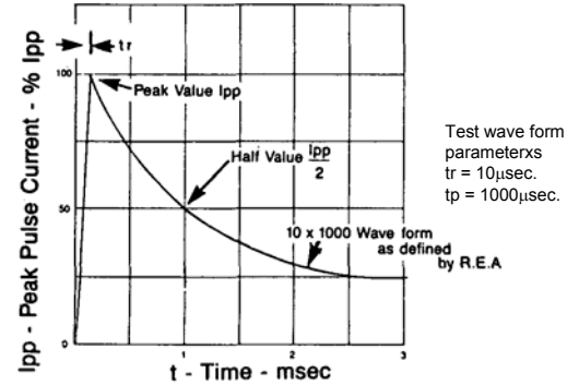
FIGURE 2 – PULSE WAVEFORM
