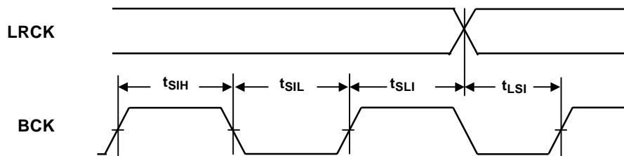
Fig.4 BCK, LRCK Timing Diagram
