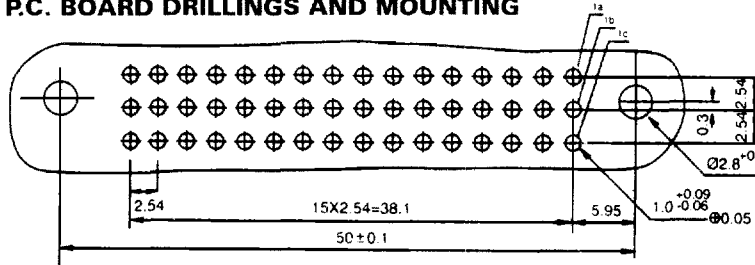
P.C. BOARD DRILLINGS AND MOUNTING
