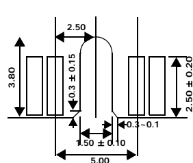
Detail of Contacts D
