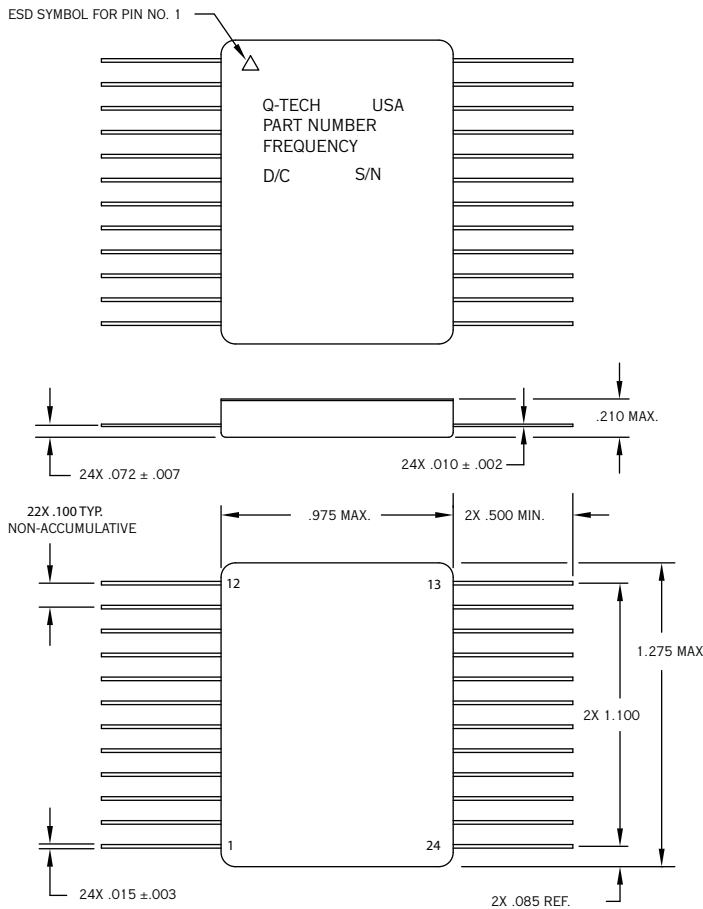
FIGURE 1 INTERFACE CONTROL DRAWING 24 pin Flat-Pack
