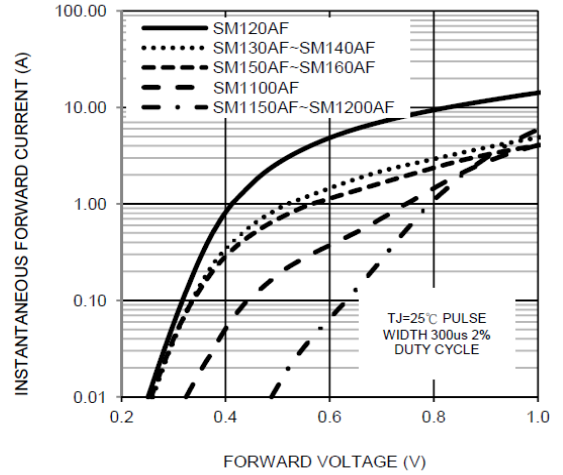
FIG. 2-TYPICAL FORWARD CHARACTERISTICS
