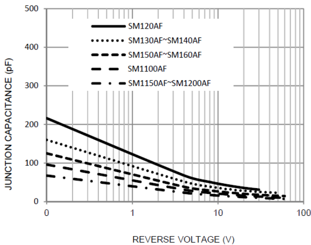
FIG. 5-TYPICAL JUNCTION CAPACITANCE
