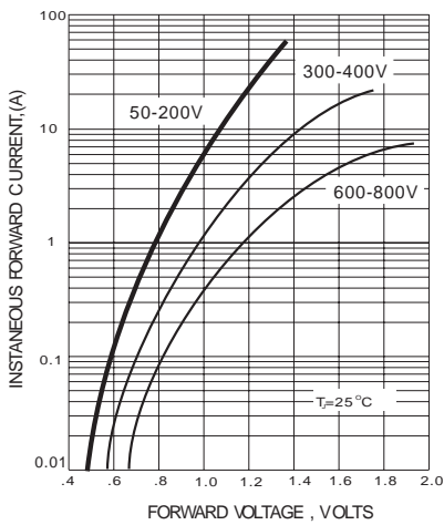
Fig.2- FORWARD CHARACTERISTICS
