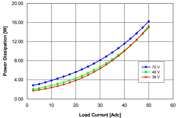
Fig. 4: Power dissipation vs. load current and input voltage for converter mounted vertically with air flowing from pin 3 to pin 1 at a rate of 300 LFM (1.5 m/s) and Ta = 25°C.
