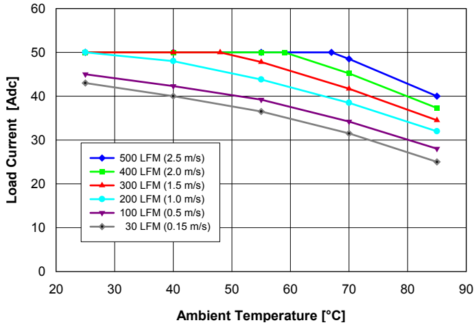
Fig. 1: Available load current vs. ambient air temperature and airflow rates for QM48T50018 converter with B height pins mounted vertically with air flowing from pin 3 to pin 1, MOSFET temperature ≤ 120°C, Vin = 48 V.
