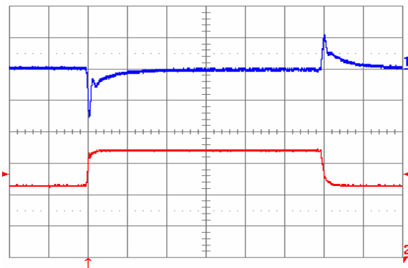
Fig. 7: Output voltage response to load current step-change (22.5 A – 33.75 A – 22.5 A) at V_{in} = 48\text{ V} . Top trace: output voltage (100 mV/div.). Bottom trace: load current (10 A/div.). Current slew rate: 1 A/ \mu\text{s} . C_o = 470\text{ }\mu\text{F} tantalum + 1 \mu\text{F} ceramic. Time scale: 0.2 ms/div.
