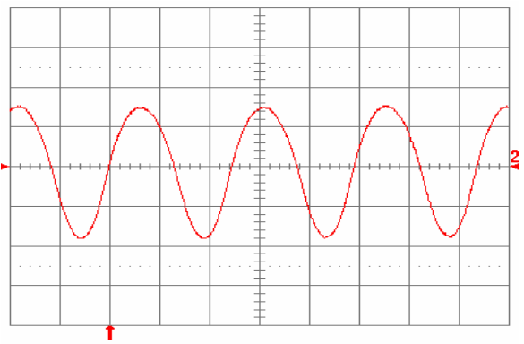
Fig. 11: Input reflected ripple current, i_c (100 mA/div), measured at input terminals at full rated load current and V_{in} = 48 V. Refer to Fig. 9 for test setup. Time scale: 1 \mu s/div.
