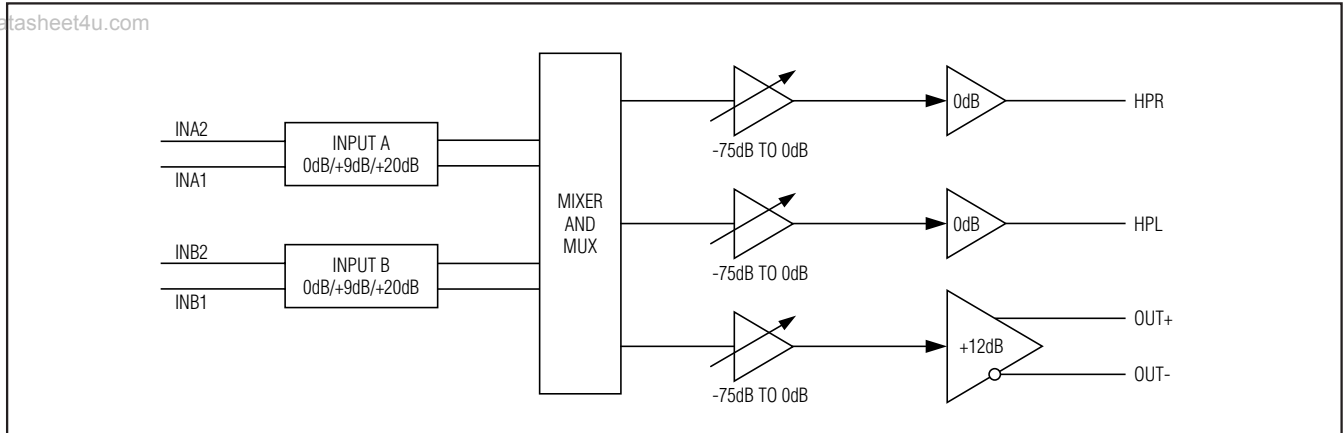
Figure 1. Signal Path
