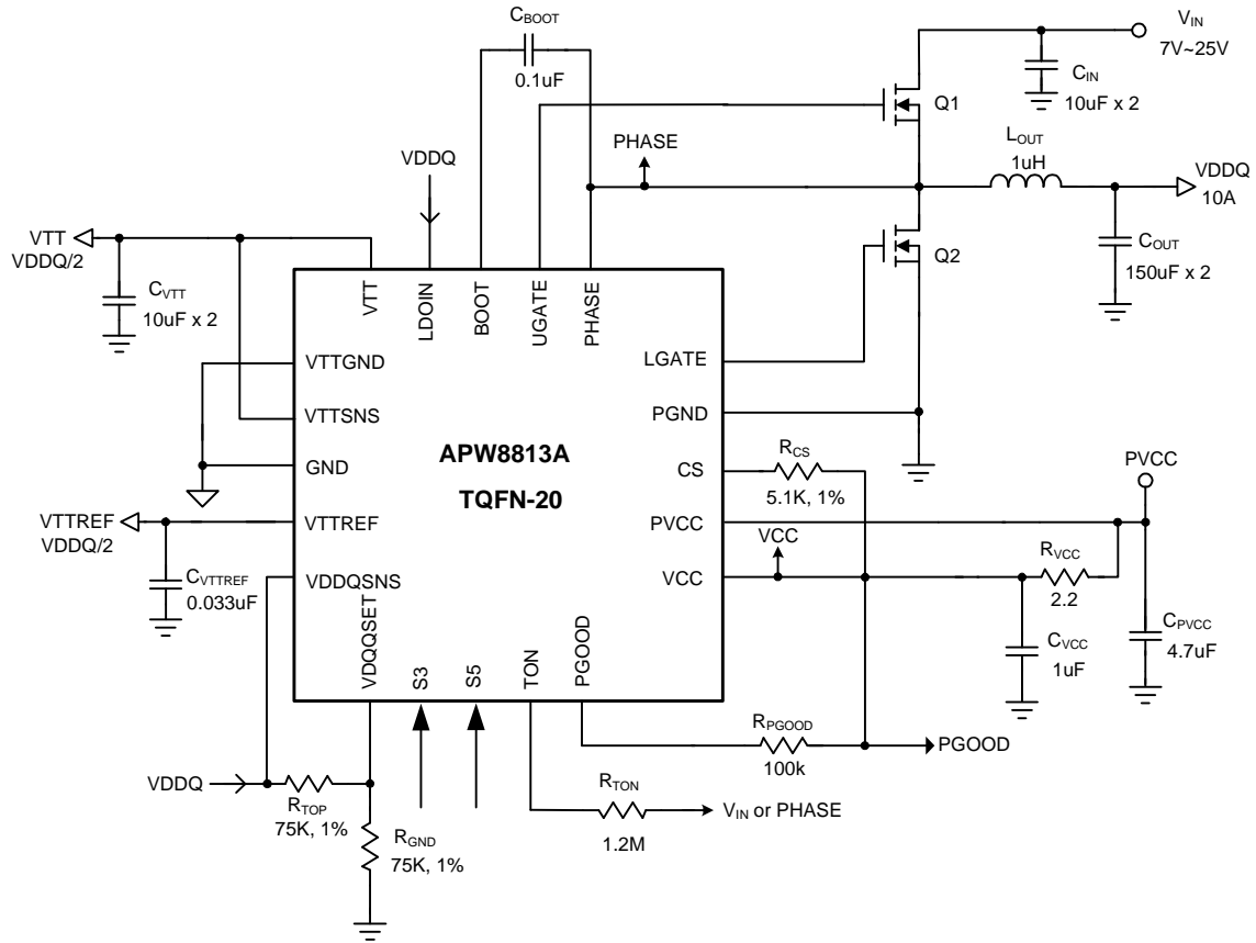
VDDQ=Adjustable, External LDOIN
