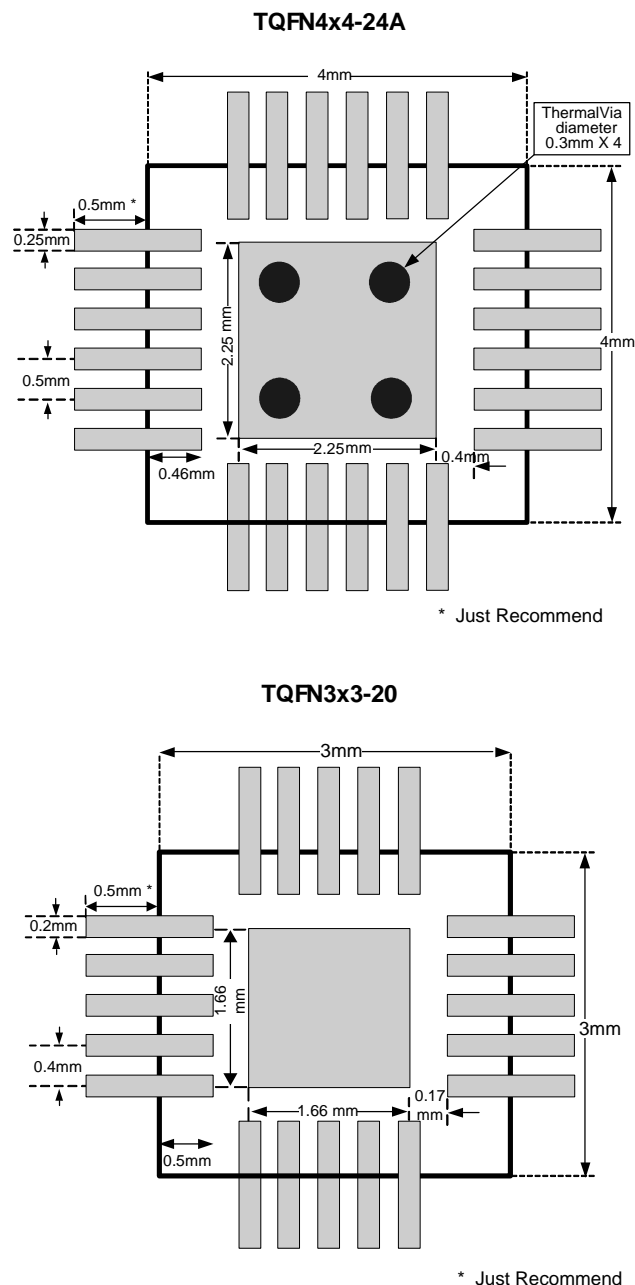
Figure 3. Recommended Minimum Footprint
