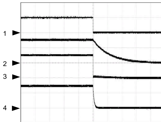
S5 Shutdown- Non-Tracking Discharge
