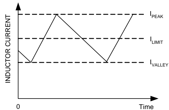
Figure 2. Current-Limit Algorithm
