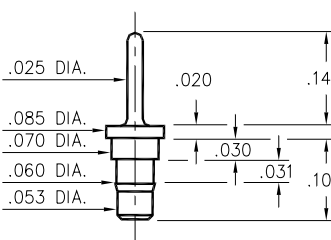
0940-0-00-XX-00-00-03-0 Press-fit in .057 mounting hole
