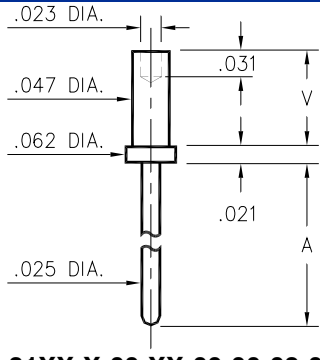
31XX-X-00-XX-00-00-08-0 Swage mount in .052 hole
