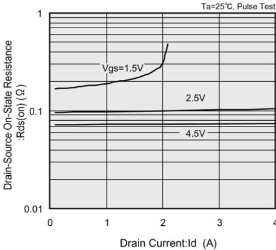
(4) Drain-Source On-State Resistance vs. Drain Current
