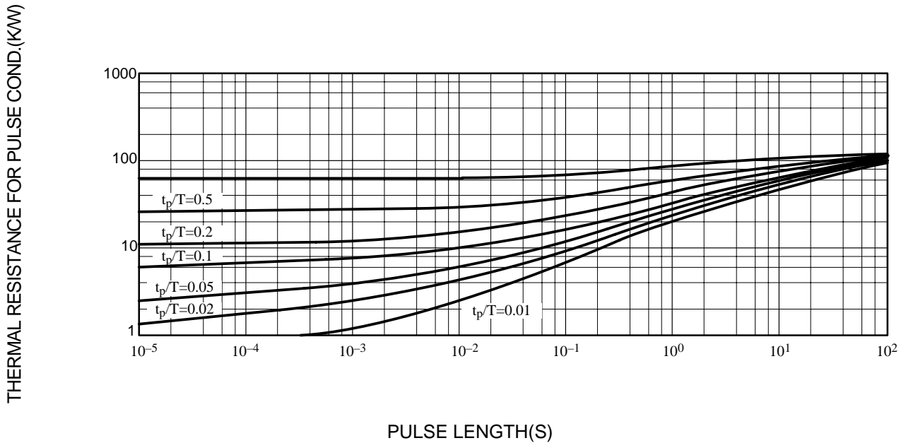
FIG.3 – THERMAL RESPONSE
