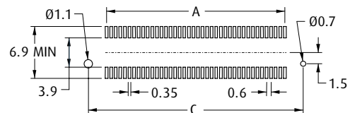
Recommended PC Board Pattern
