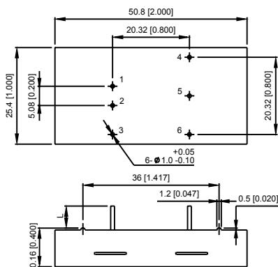
Unit: mm[inch]
