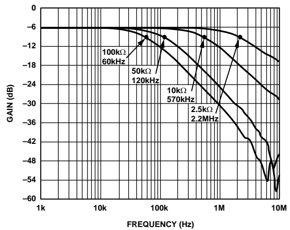
Figure 20. -3\text{ dB} Bandwidth at Code = 0x80
