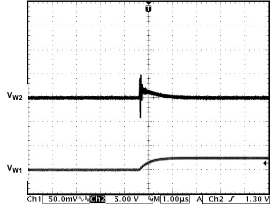
Figure 24. Analog Crosstalk
