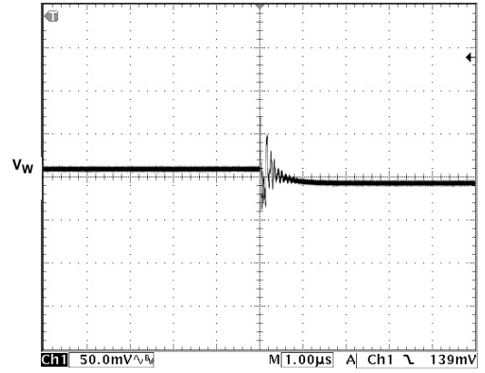
Figure 25. Midscale Glitch, Code 0x80 to Code 0x7F
