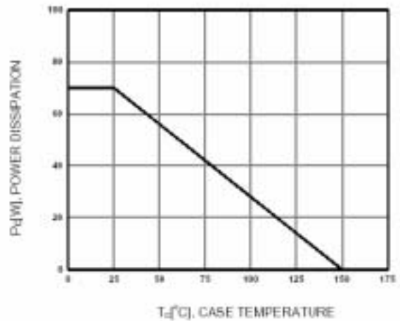
Figure 4. Power Derating
