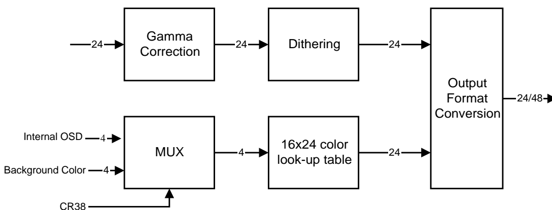
Figure 10 OSD color look-up table data path diagram
