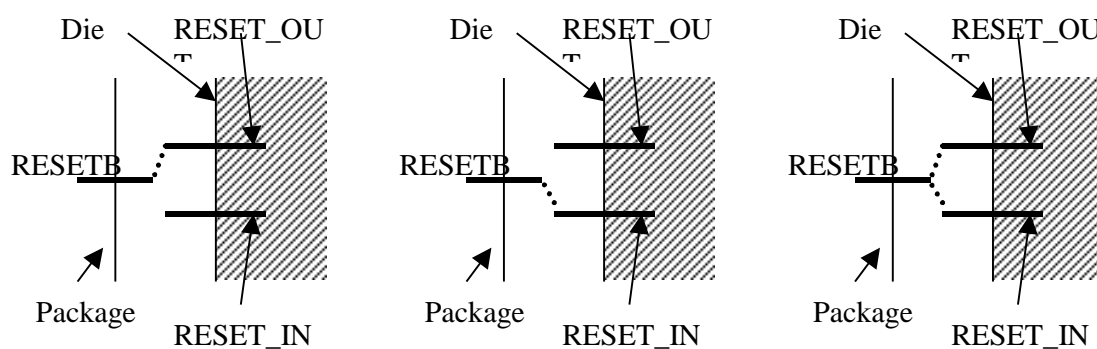
Figure 17 Three kinds of RESET function
