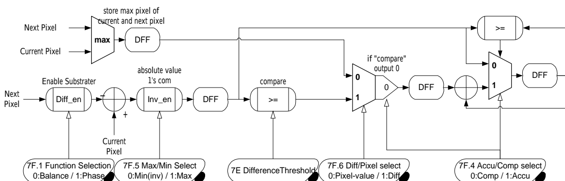
Figure 14 Auto-Tracking Control Block
