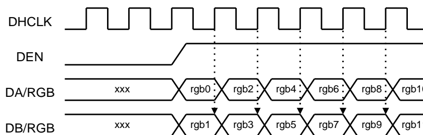
Figure 7 Double Pixel Mode Display Data Timing
