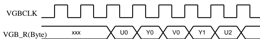
Figure 4 Input YUV 4:2:2(8-bits) Timing
