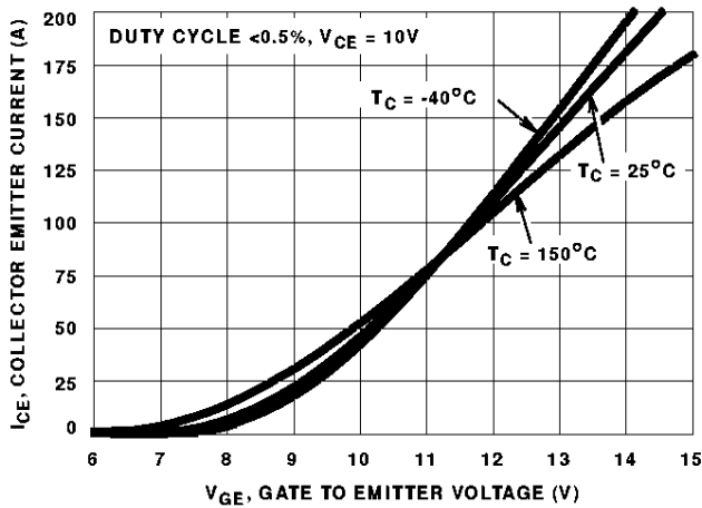
FIGURE 1. TRANSFER CHARACTERISTICS
