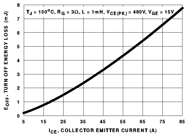
FIGURE 10. TURN OFF ENERGY LOSS AS A FUNCTION OF COLLECTOR EMITTER CURRENT
