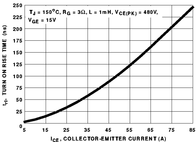
FIGURE 7. TURN ON RISE TIME AS A FUNCTION OF COLLECTOR EMITTER CURRENT
