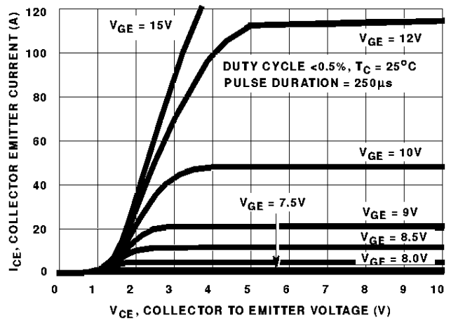
FIGURE 2. SATURATION CHARACTERISTICS
