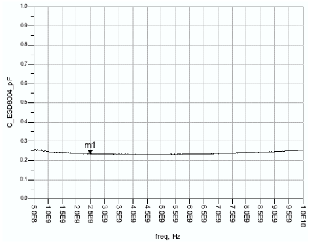
Figure 10. Junction Capacitance; V R = 0 V, f = 500 MHz – 10 GHz
