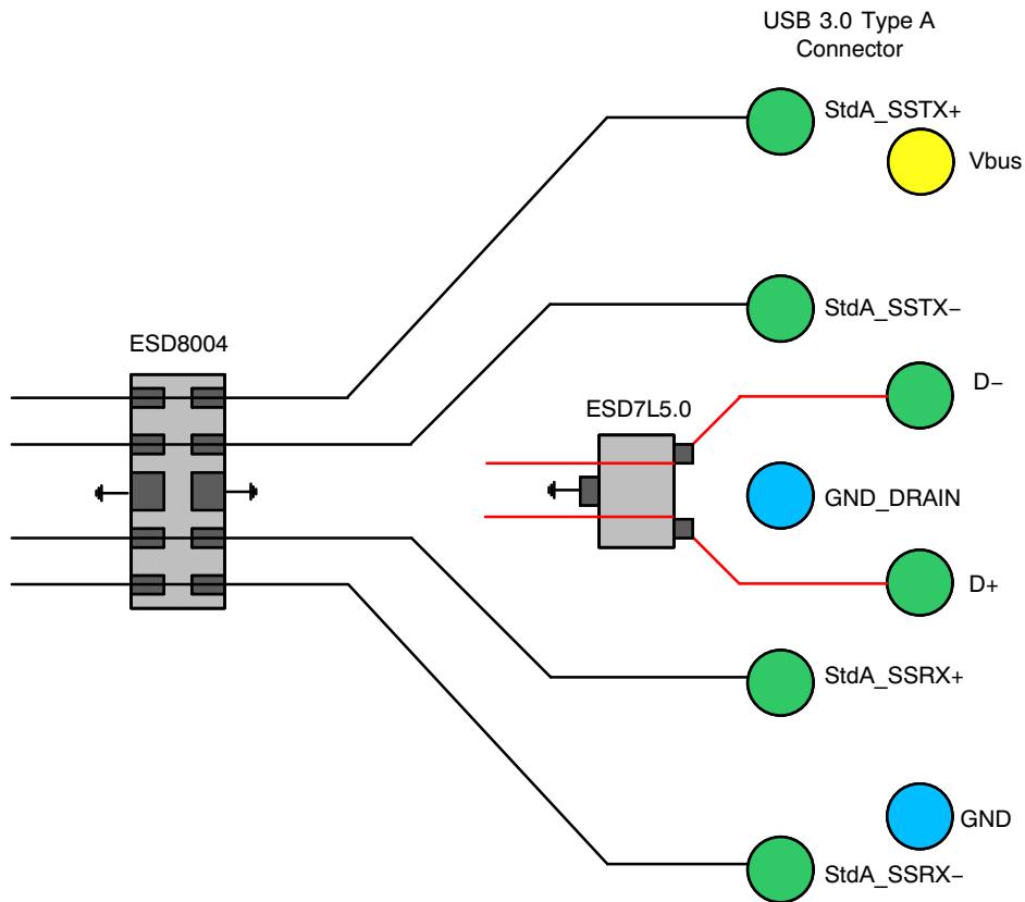
Figure 13. USB3.0 Layout Diagram
