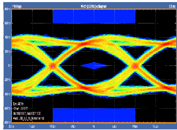
Figure 11. USB3.0 Eye Diagram with and without ESD8004. 5 Gb/s
