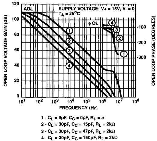
FIGURE 19. OPEN-LOOP RESPONSE
