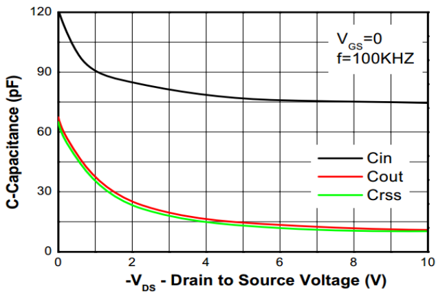
Capacitance
