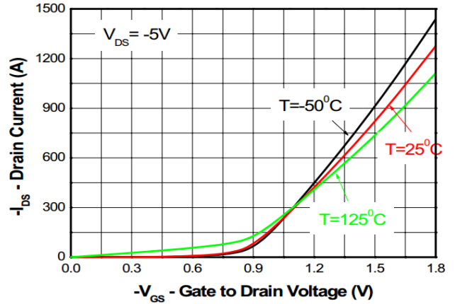
Transfer characteristics
