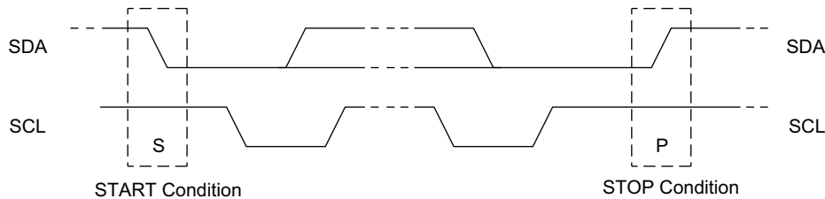
Figure 4. Data Transfer on the I 2 C Bus
