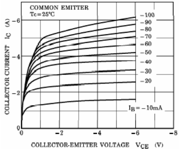
Fig.4 Static Characteristic
