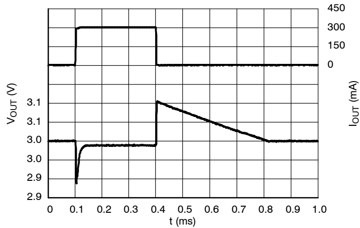
Figure 70. Load Transients, 3.0 V Version, I OUT = 1 – 300 mA, t R = t F = 0.5 μs, V IN = 6.0 V, ECO = H
