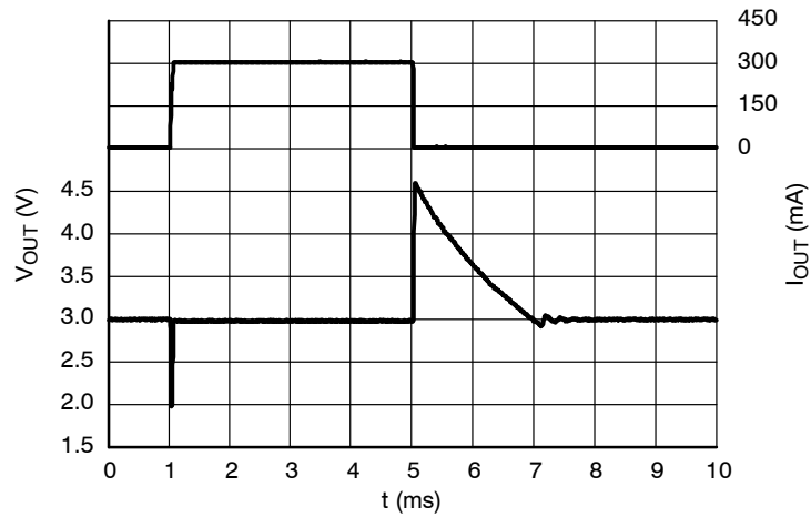
Figure 69. Load Transients, 3.0 V Version, I OUT = 1 – 300 mA, t R = t F = 0.5 μs, V IN = 6.0 V, ECO = L
