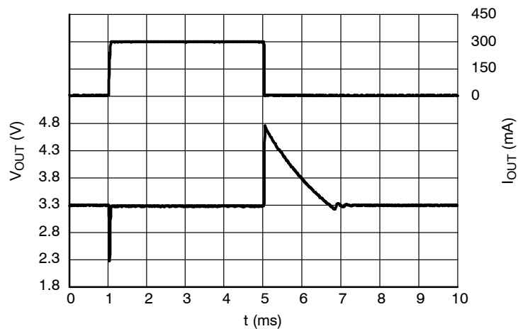
Figure 71. Load Transients, 3.3 V Version, I OUT = 1 – 300 mA, t R = t F = 0.5 μs, V IN = 6.3 V, ECO = L
