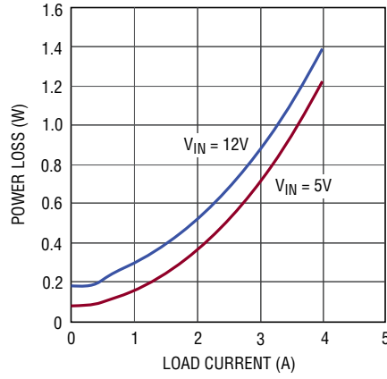
Figure 7. 1.5V Loss
