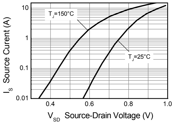
Reverse Diode Characteristic
