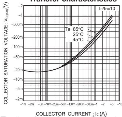
C-E saturation voltage vs. Collector current
