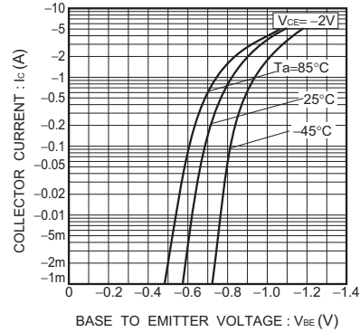
Transfer characteristics
