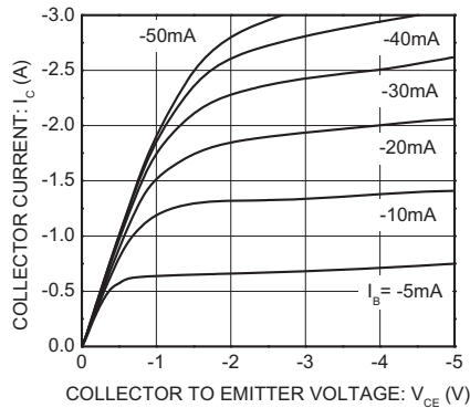
Output characteristics
