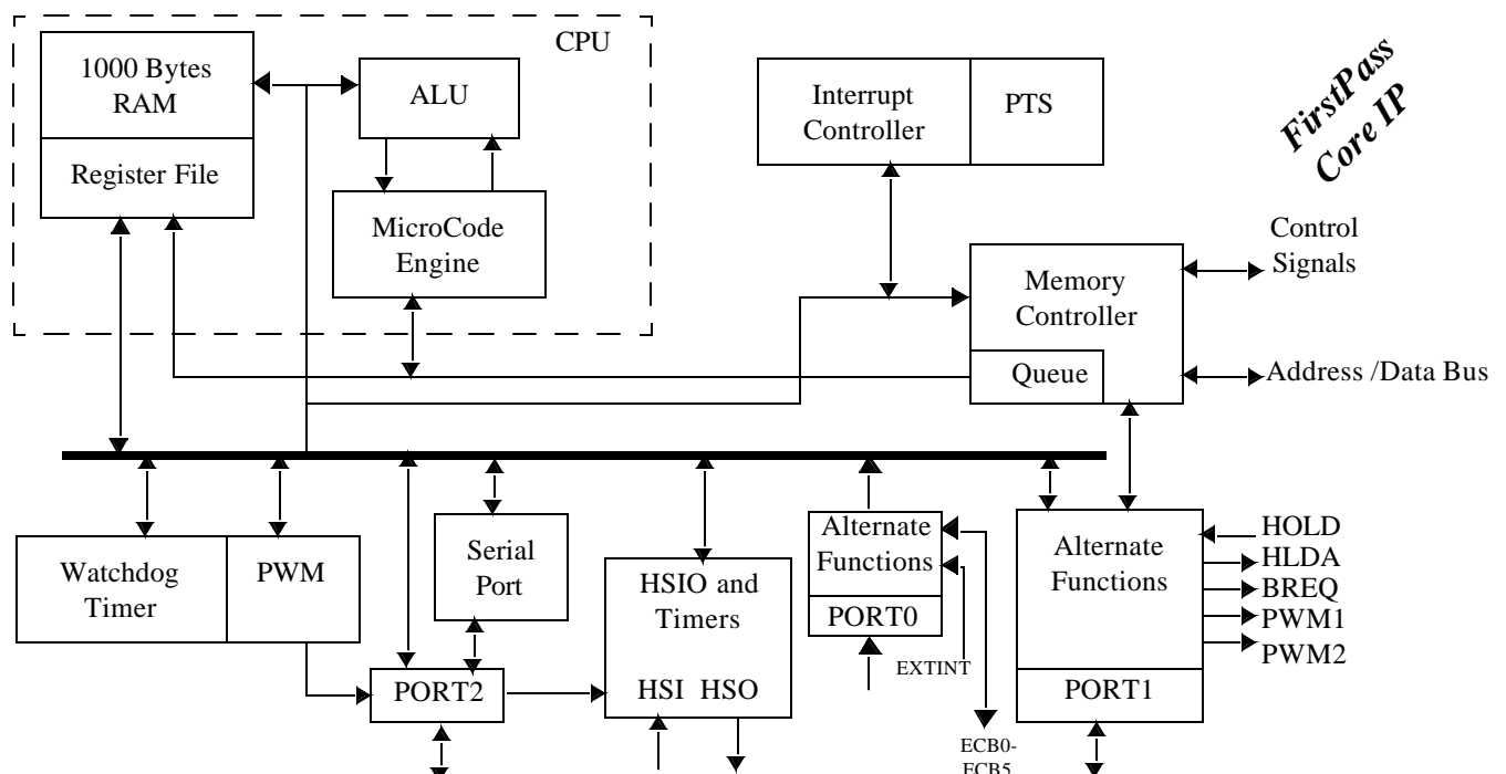
Figure 1. UT80CRH196KDS Microcontroller
