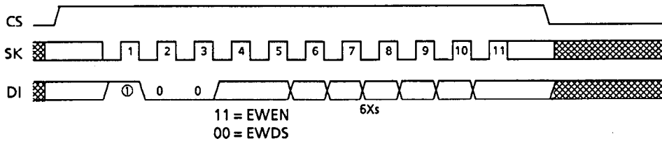
Figure 14 EWEN/EWDS Timing (S-29L220A)
