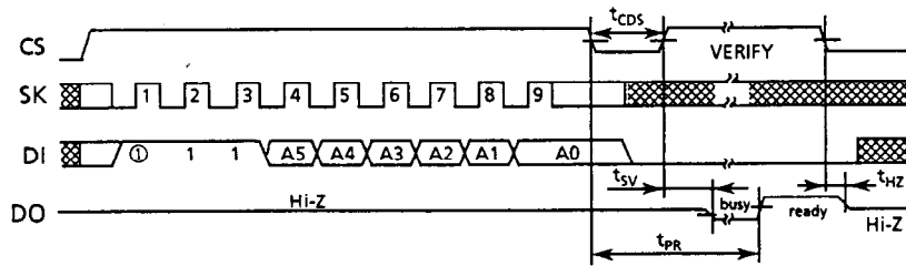
Figure 10 ERASE Timing (S-29L130A)
