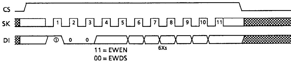
Figure 15 EWEN/EWDS Timing (S-29L330A)
