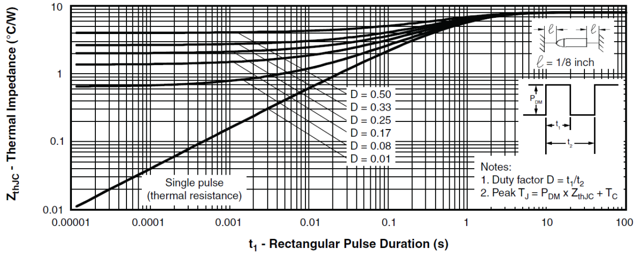
Fig. 4 - Maximum Thermal Impedance Z_{thJL} Characteristics
