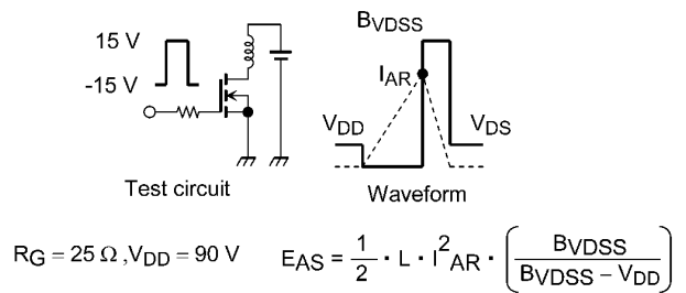
Fig. 8.16 Test Circuit/Waveform
