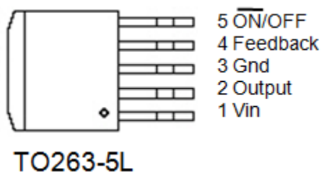
Figure 2. Pin Configuration of EC9301H
