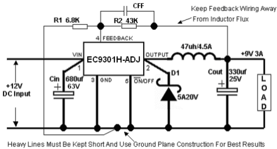
Figure 12. Typical Application of EC9301H For ADJ
