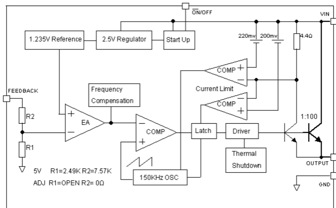
Figure 3 Function Block Diagram of EC9301H
