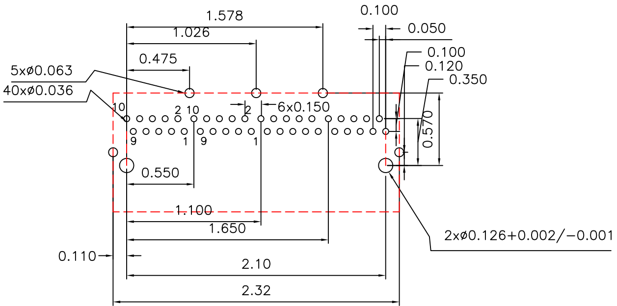
Four Port Suggested Footprint: (Top View)
