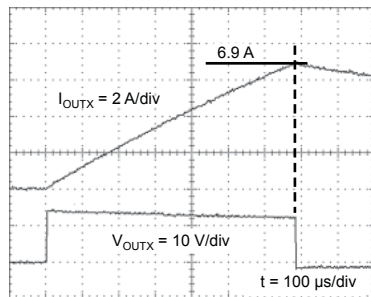
High-side DMOSFET OCP Operation Example
