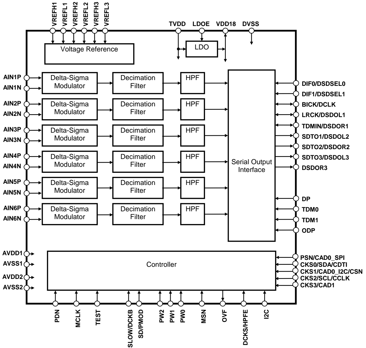
Figure 1. Block Diagram
