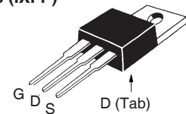
TO-220 (IXFP)
