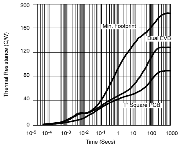
FIGURE 4. Dual 1206-8 ChipFET
