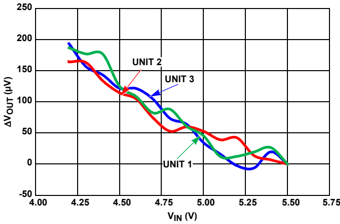
FIGURE 123. LINE REGULATION, THREE UNITS
