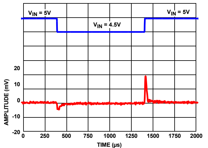
FIGURE 7. LINE TRANSIENT RESPONSE WITH 10\mu F LOAD
