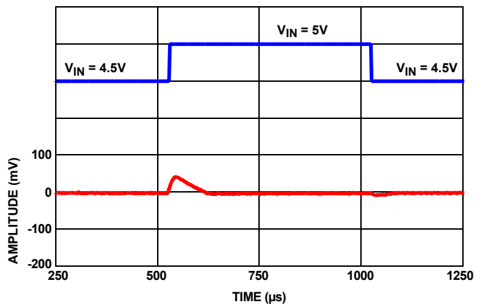
FIGURE 109. LINE TRANSIENT RESPONSE WITH 10\mu F LOAD
