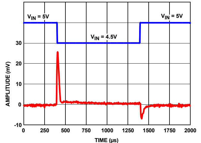
FIGURE 41. LINE TRANSIENT RESPONSE WITH 10\mu F LOAD
