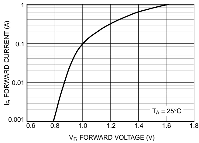
Figure 7. Forward Voltage
