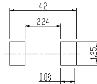
Soldering footprint
