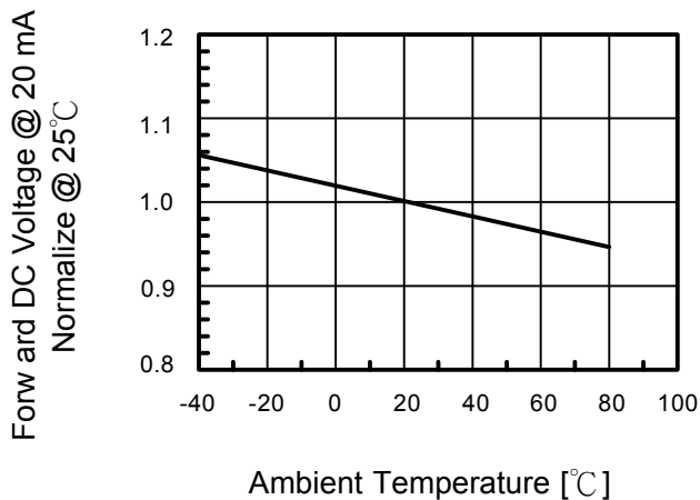
Fig.5 Forward DC Voltage vs. Temperature
