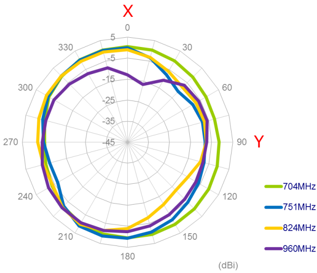
XY Plane
