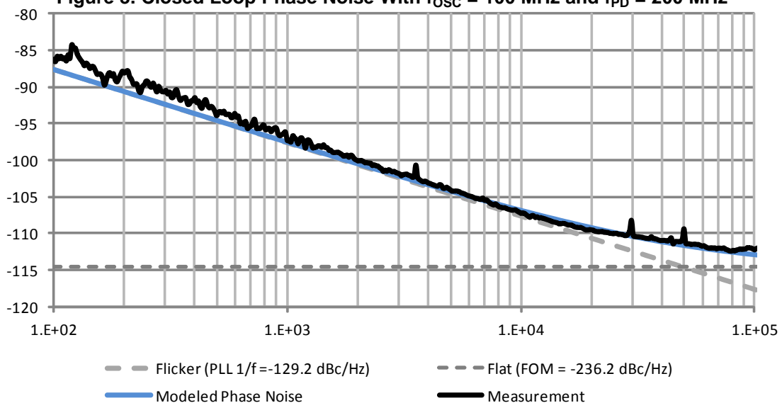
Figure 3. Closed Loop Phase Noise With f_{OSC} = 100 MHz and f_{PD} = 200 MHz
