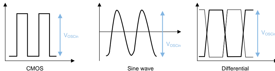
Figure 44. Input Clock Definitions
