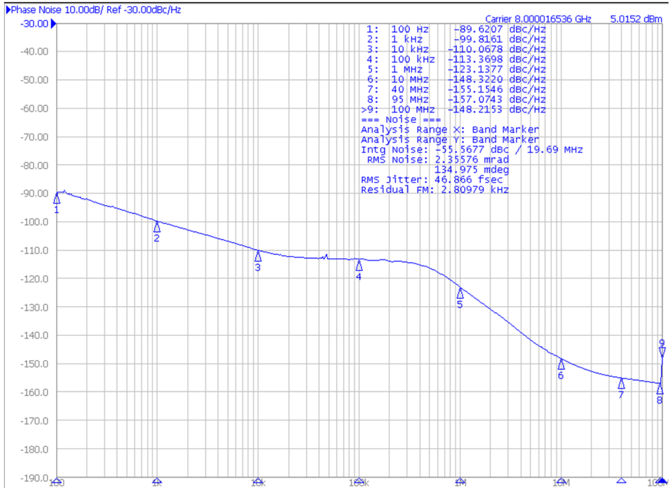
Figure 47. Typical Jitter
