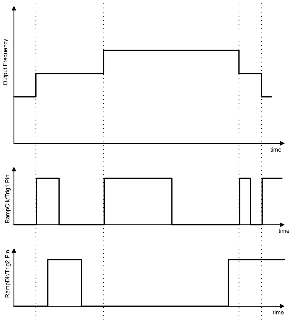
Figure 23. Step Ramping Example
