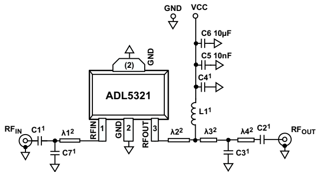
Figure 28. Basic Connections
