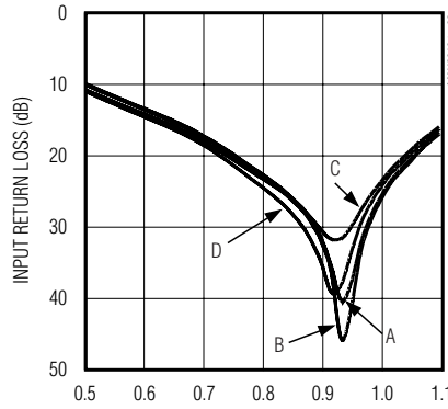
SMALL-SIGNAL INPUT RETURN LOSS vs. FREQUENCY
